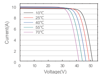
Current-Voltage Curve JAM72S12-385/PR/1000V
